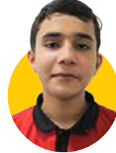
NIRYANK MANARIYA 94.60%
