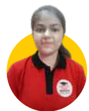
ANUSHKA RAJPUT 97.80%
